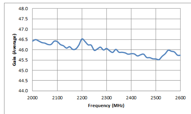
Gain
