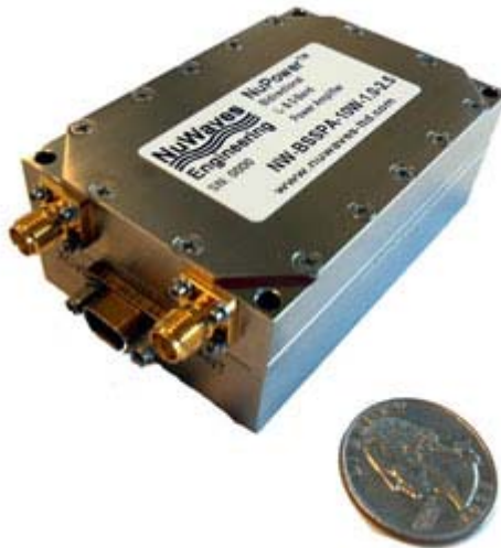
Figure 1. NuWaves' NuPower Xtender™ features 10 W of RF output power and a 3.5 dB noise figure.
