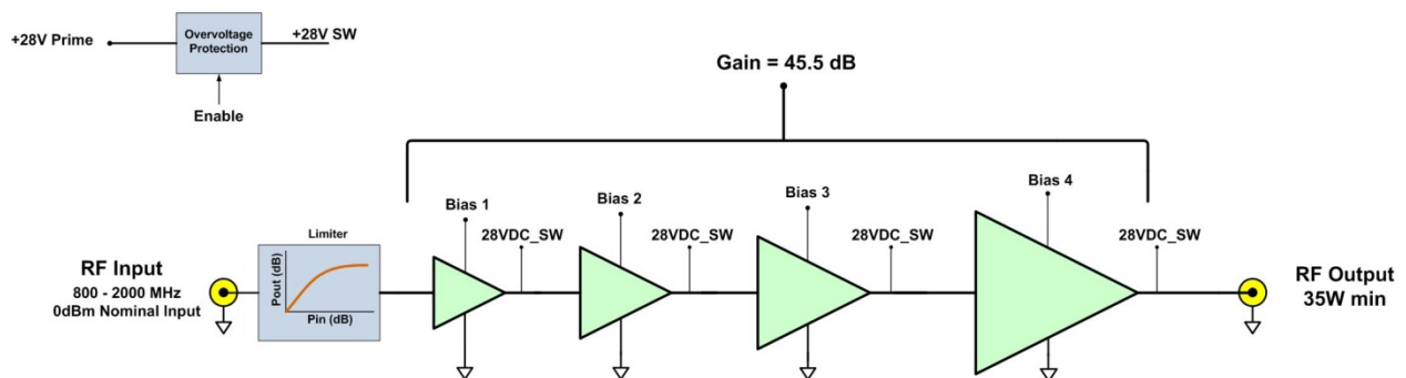
Figure 1: NuPower 13G05A Functional Diagram
