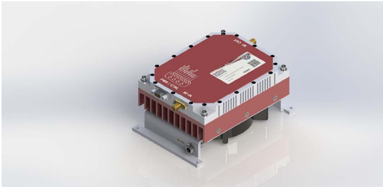
Figure 3: The NuPower PA Kit offers “out-of-the-box” operation for the user. The 28 VDC fan-cooled heatsink is shown with the NuPower 13G05A mounted.
