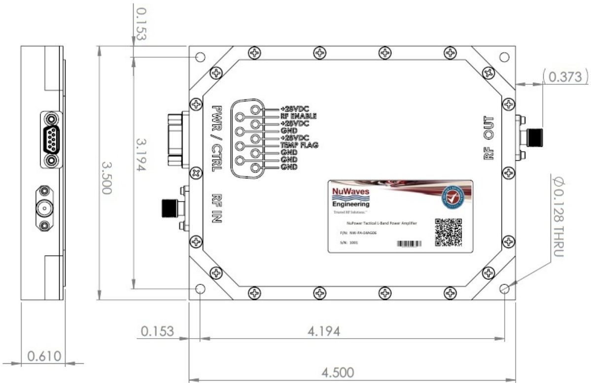
Figure 2: NuPower 13G05A Mechanical Outline
